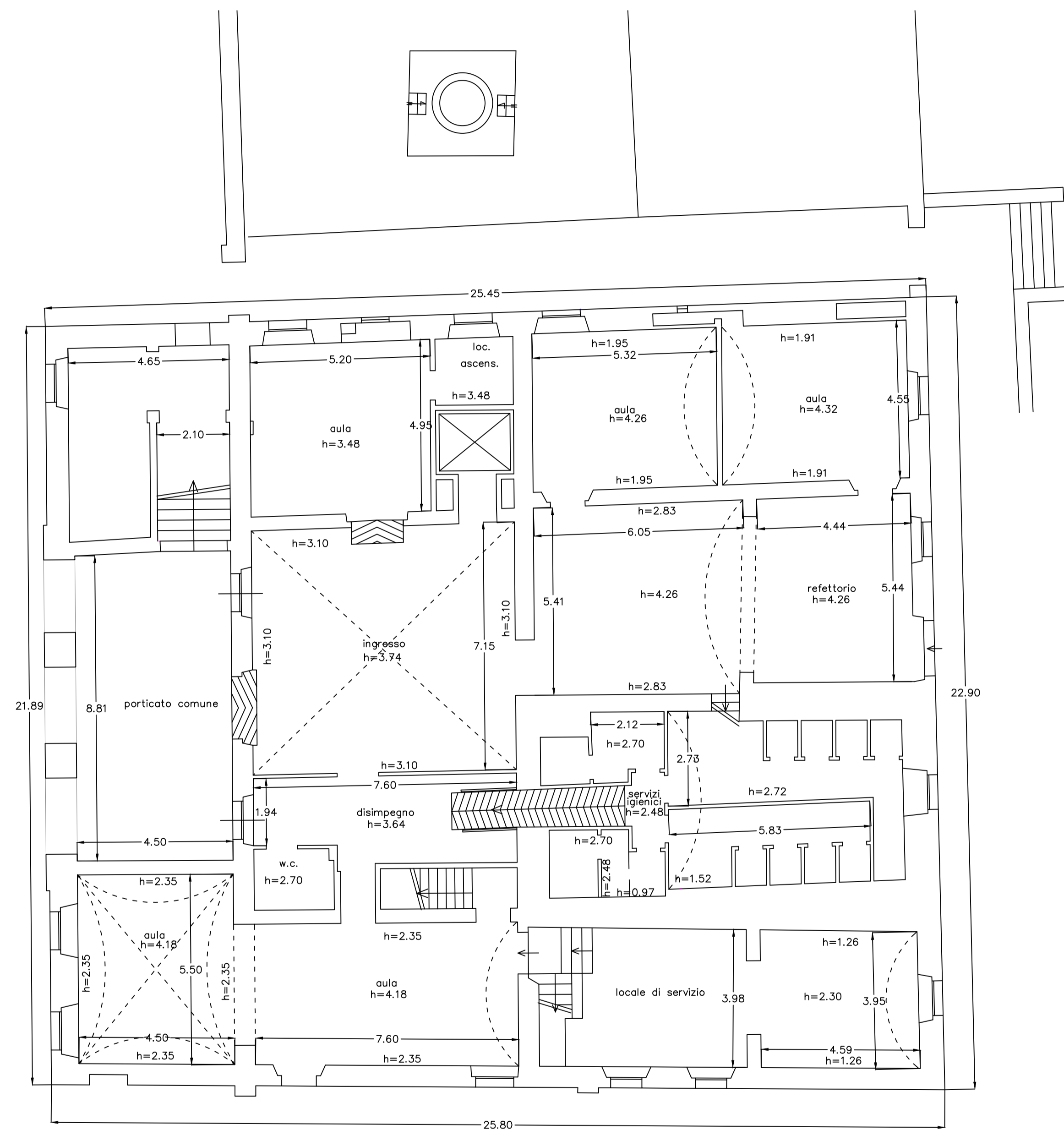
PIANO TERRA scala 1:100
